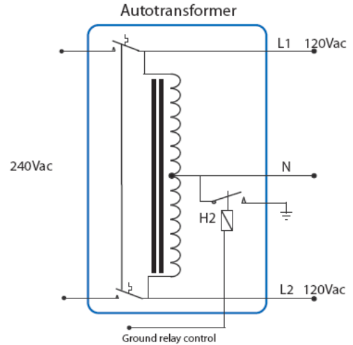
Autotransformer: schematic diagram
