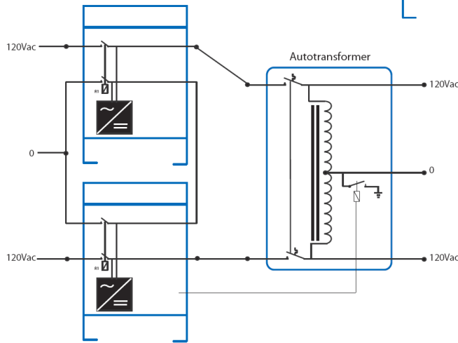
Step-Up: 120VAC to 240VAC (Internal ground relay of inverter/charger may be used)
